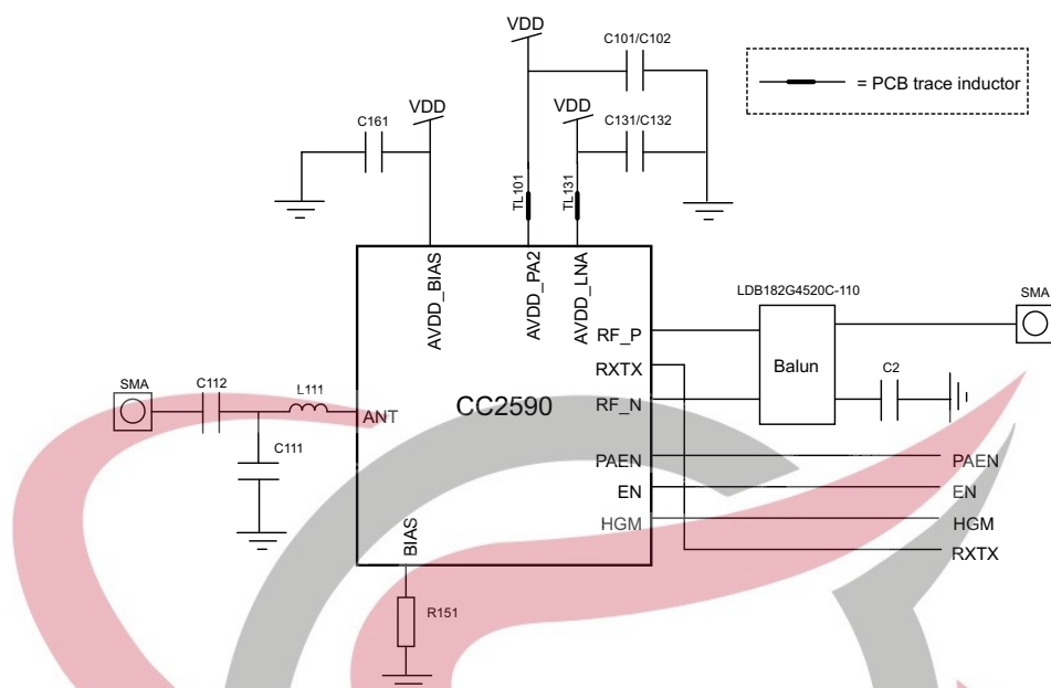
Figure 2. CC2590EM Evaluation Module
